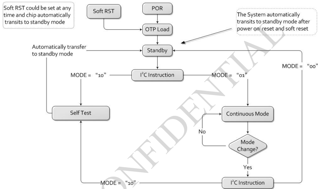
Figure 9. Modes Transition
